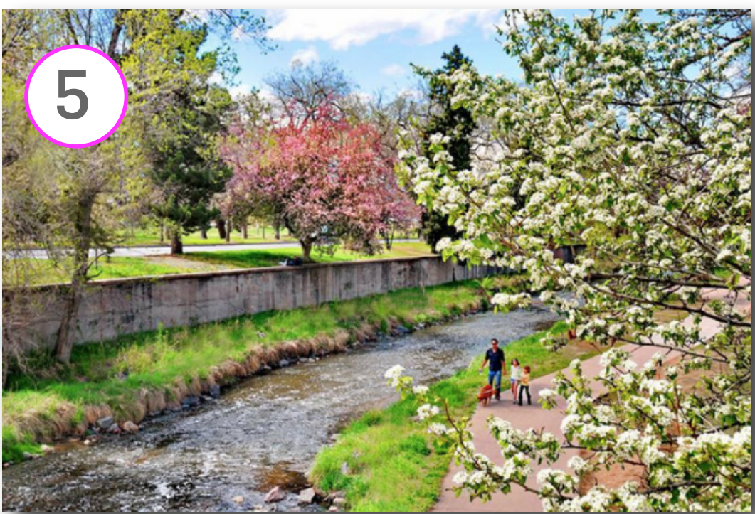
daylighted stream
