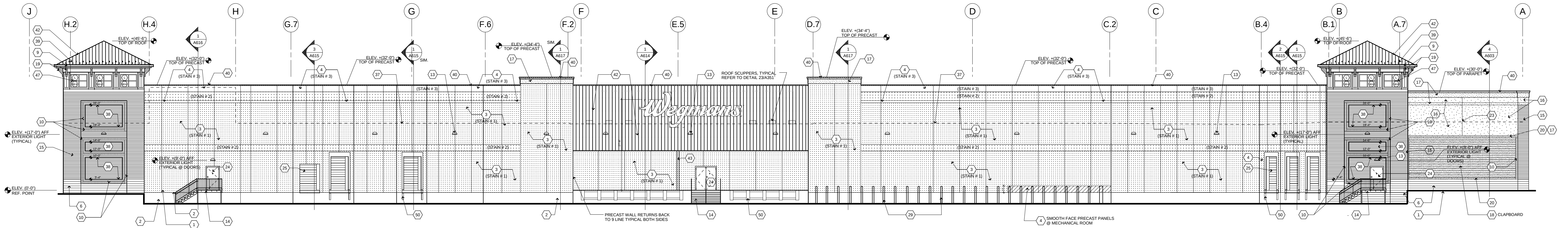
REAR (SOUTH) ELEVATION
