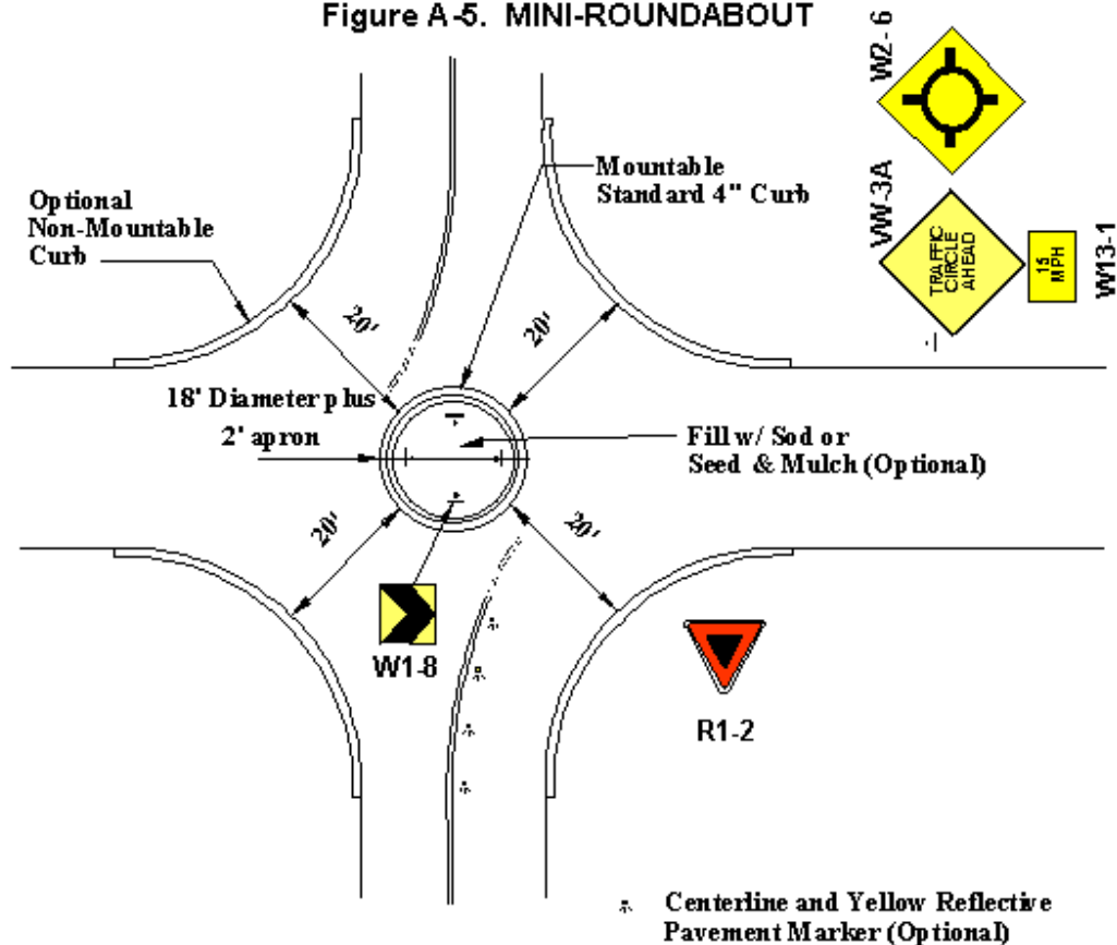
Figure A-5. MINI-ROUNDBABOUT
