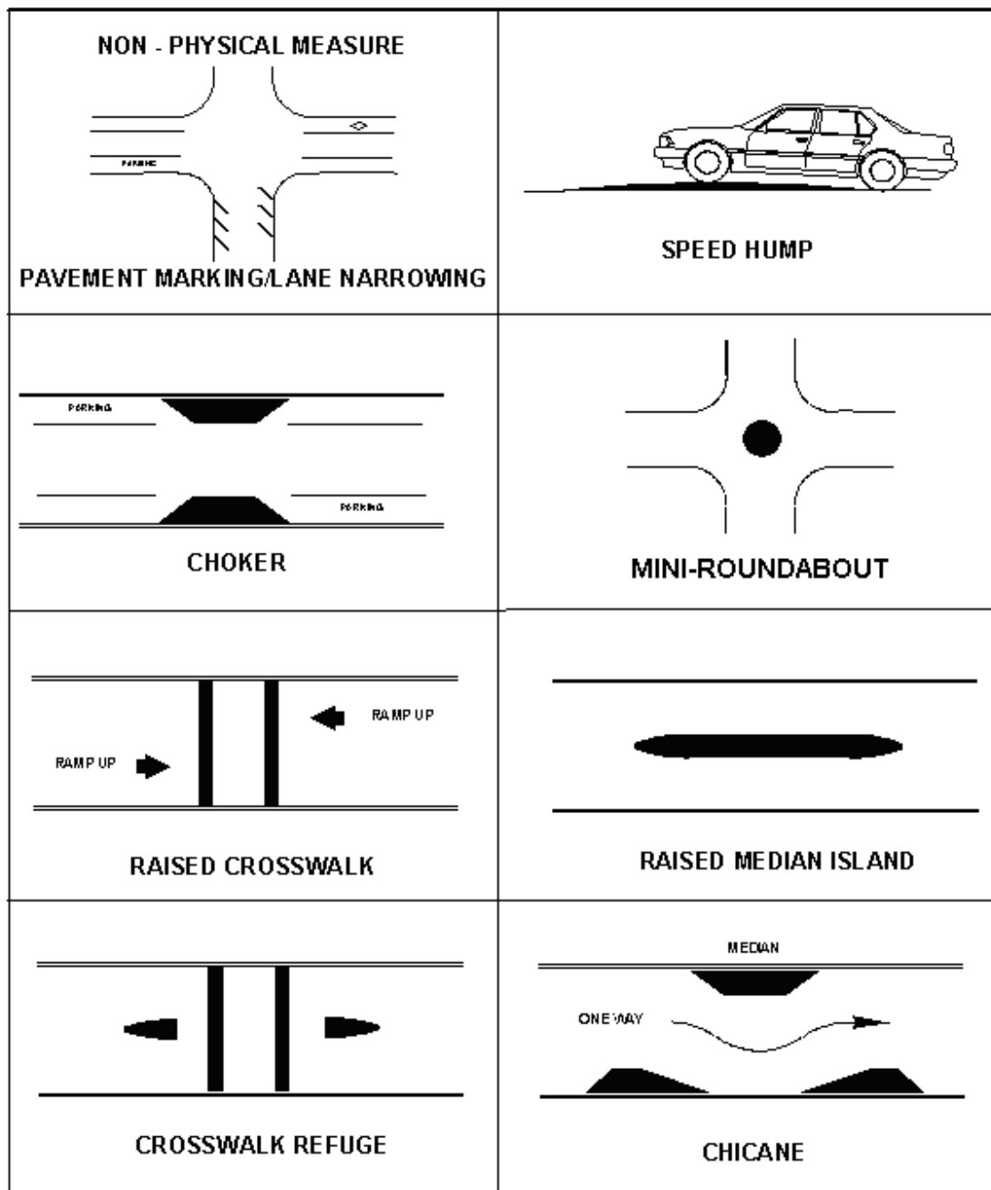
Figure 2. Typical Physical and Non-Physical Traffic Calming Measures
