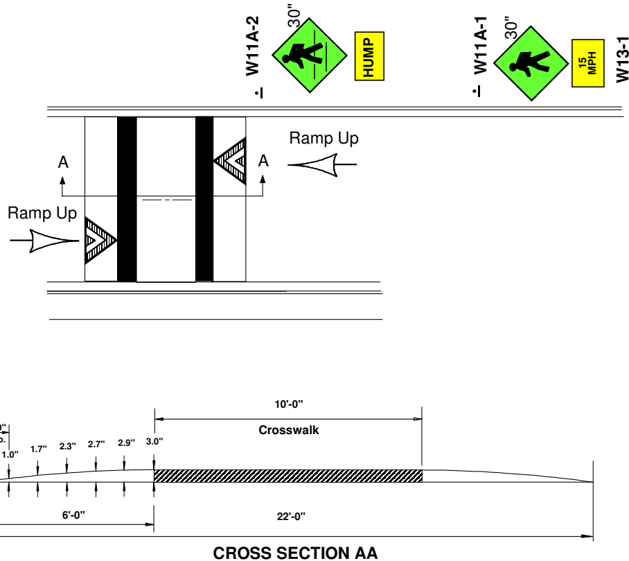
Figure A-4. RAISED CROSSWALK
