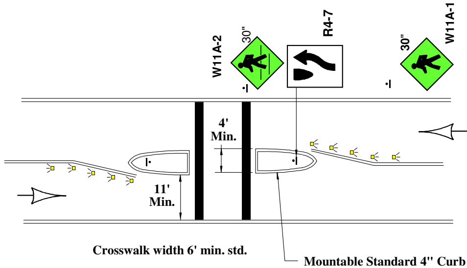
Figure A-6. CROSSWALK REFUGE
