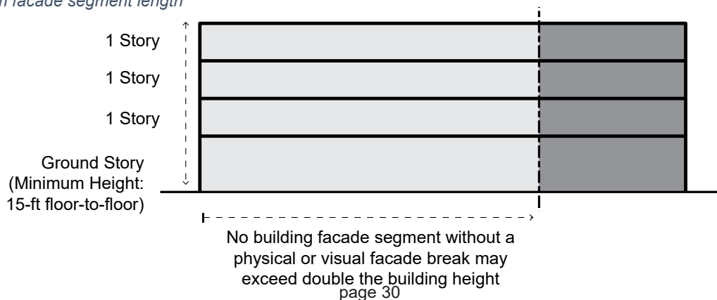
Figure 9: Maximum facade segment length
