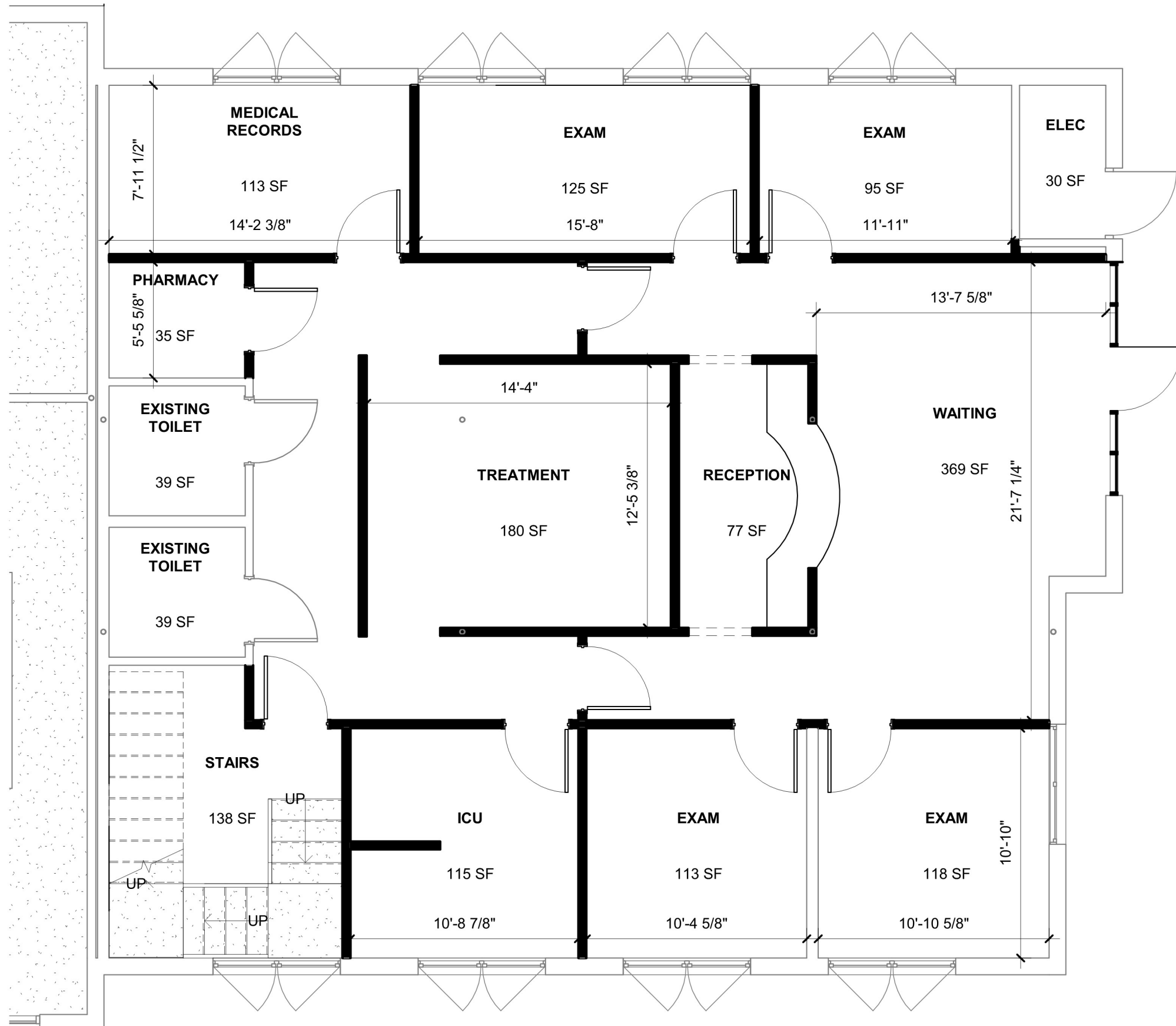
1 GROUND FLOOR PLAN 3/16" = 1'-0"
