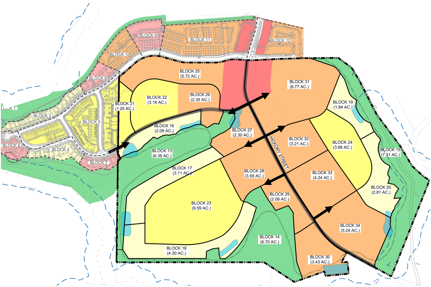
Figure 4: Proposed Phase 2 Regulating Block Plan in Context
