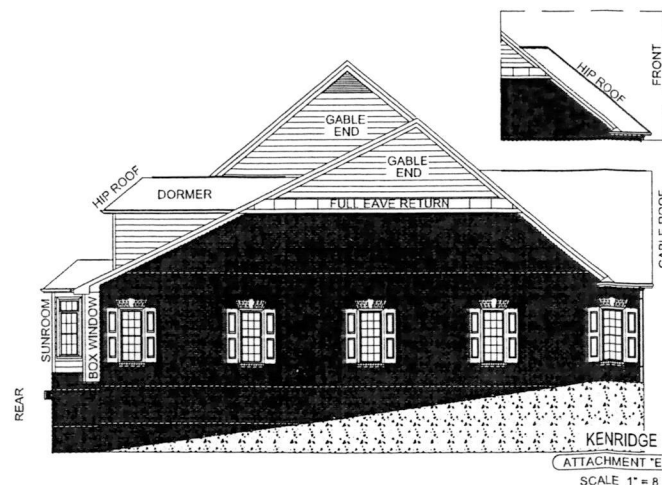
SIDE ELEVATION
