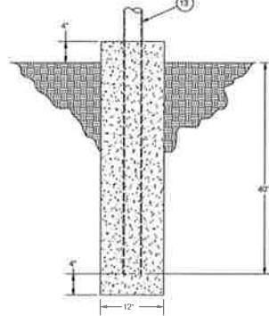
DIRECT BURIAL FOOTING
